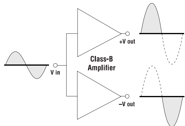
Class-B Operation
